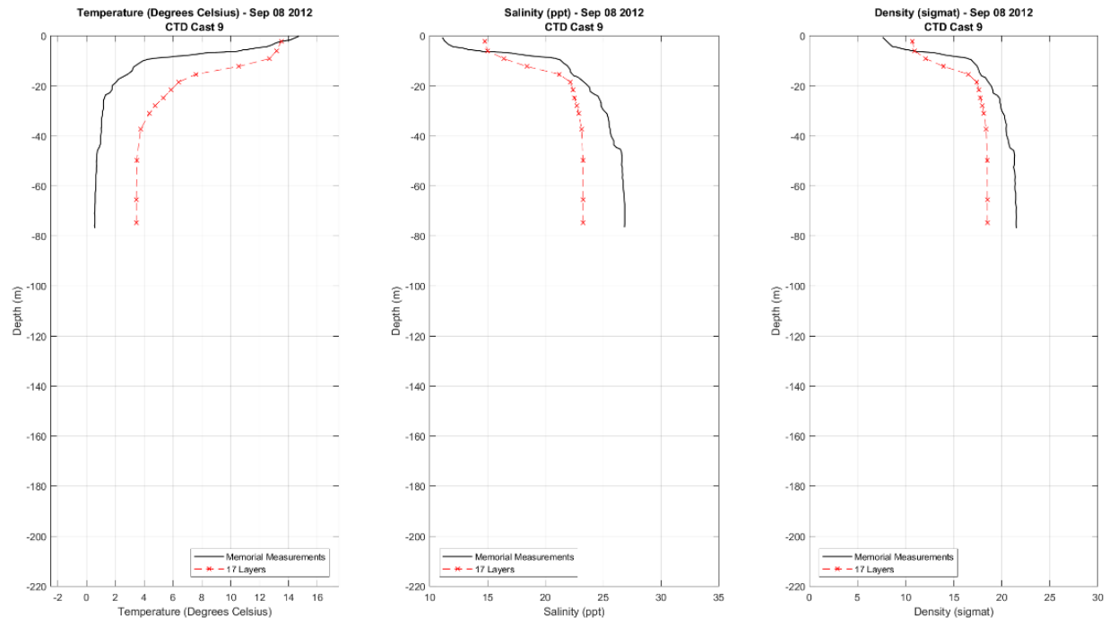
Figure 6 Comparison of measured-modelled temperature, salinity and density in west Lake Melville (CTD9)
