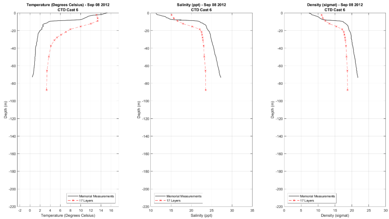
Figure 7 Comparison of measured-modelled temperature, salinity and density in central Lake Melville (CTD6)
