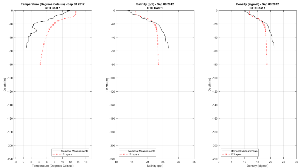
Figure 8 Comparison of measured-modelled temperature, salinity and density in east Lake Melville (CTD1)
