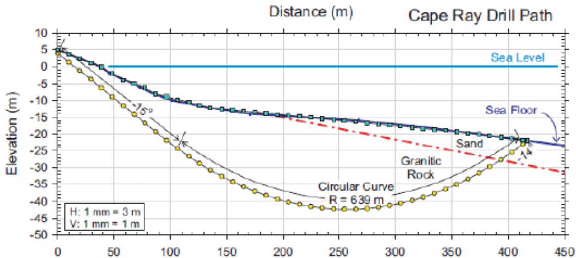
Figure 2: Cape Ray NL HDD Conceptual Design
