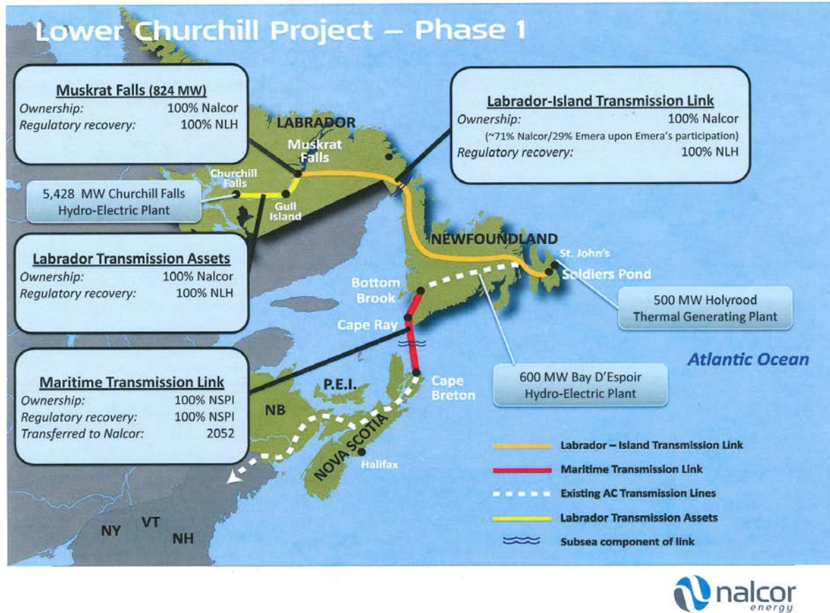
Figure 1-1 Lower Churchill Project – Phase 1 Development
