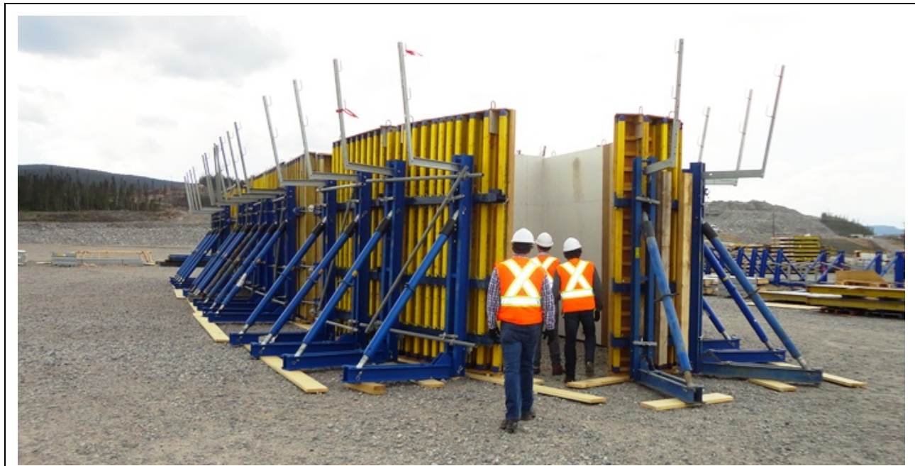
Photo 6.7: Trial assembly of tailrace pier formwork. (July 17, 2014)
