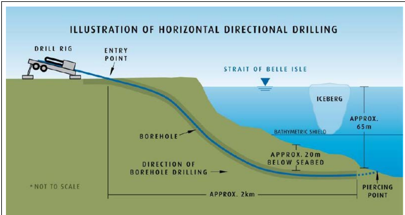
Figure 2.1: Schematic profile showing direction drilling on the shores of the Strait of Belle Isle.
