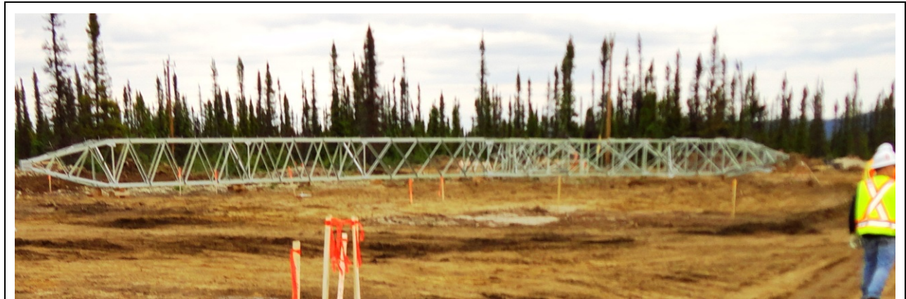
Photo 8.1: Transmission Tower Erection and Foundations. Assembled single HVac tower unit. (July 17, 2014)
