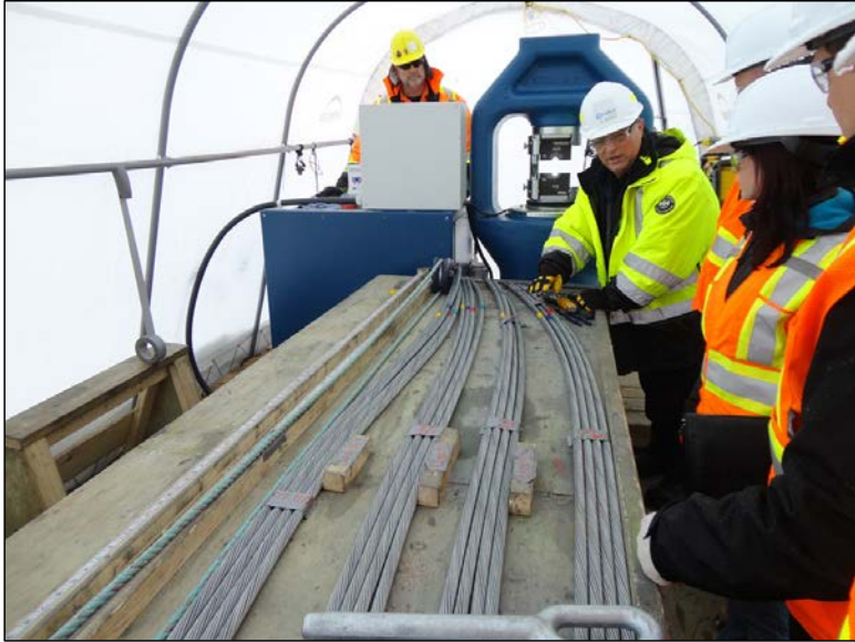
Photo 2.2: Laydown and preparation of guy cables for HVacAC transmission towers. (November 25, 2014)
